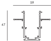
GCCX-N1000/2000/3000 Track CTN: 5 Material: Aluminum ■ Sand Black
